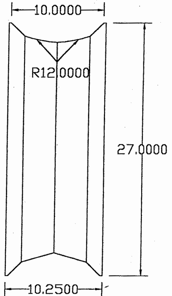
Side View
